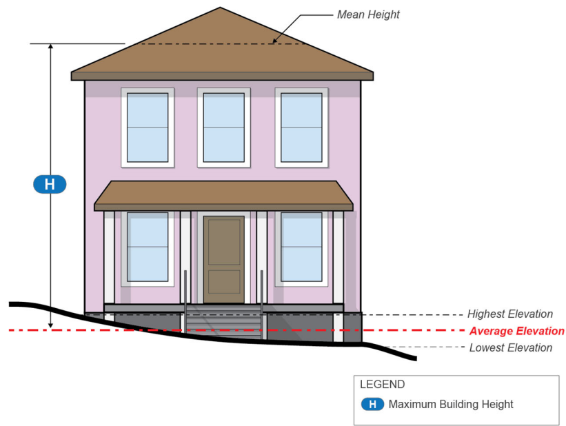
Figure 24-8 – Determining average elevation.
