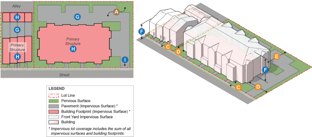
Figure 24-15 - R-20 Diagram
