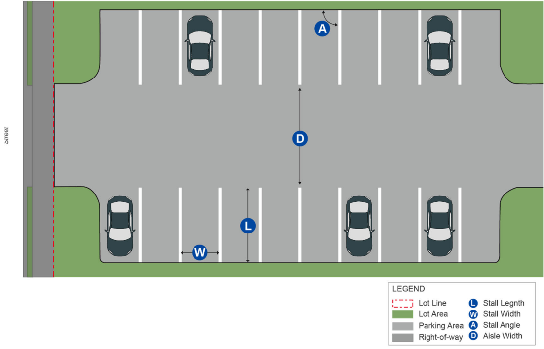
Figure 24-26 - Maneuverability standards
