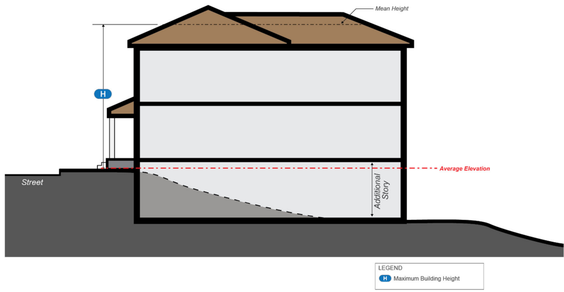
Figure 24-9 – Measurement for downward sloping sites.
